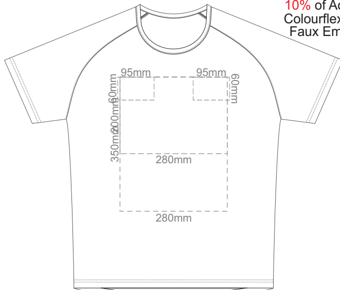
FRONT MEN'S LARGE Print area 280x200mm can be rotated to best suit.
