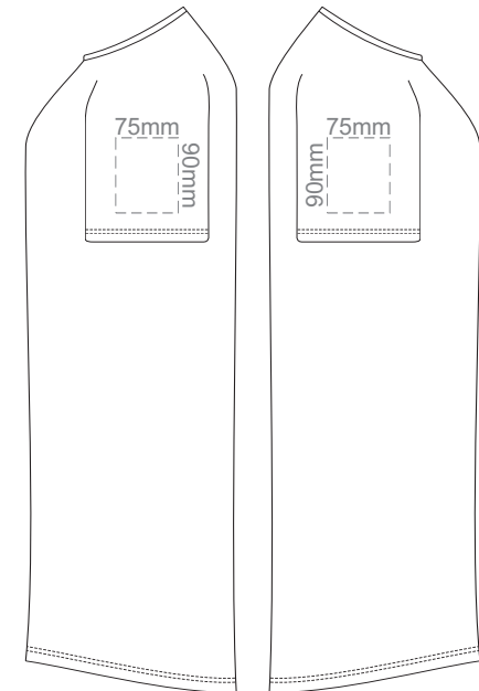
MEN'S 2XL LEFT SLEEVE
